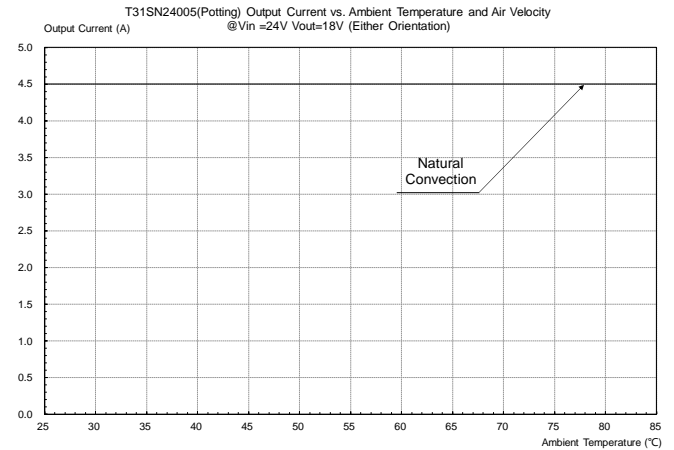
Figure 31: Output current vs. ambient temperature and air velocity @V in =24V, V out =18V (Either Orientation, Potting)
