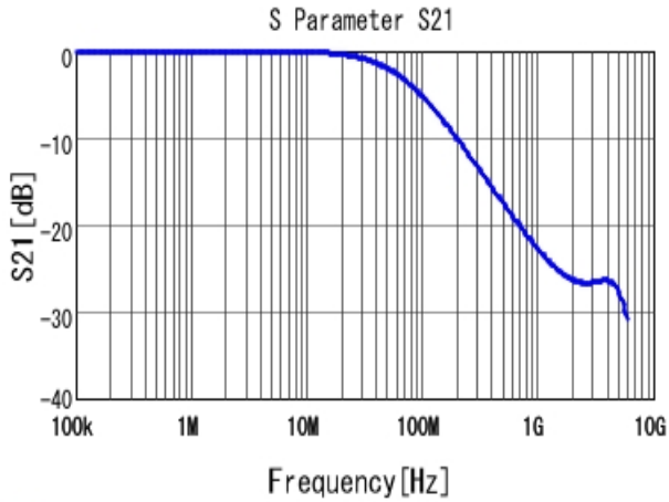
■ NFM18CC101R1C3 S21 DC0V, 25degC, Feedthrough
