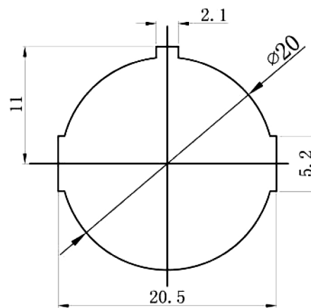
PANEL CUT-OUT
