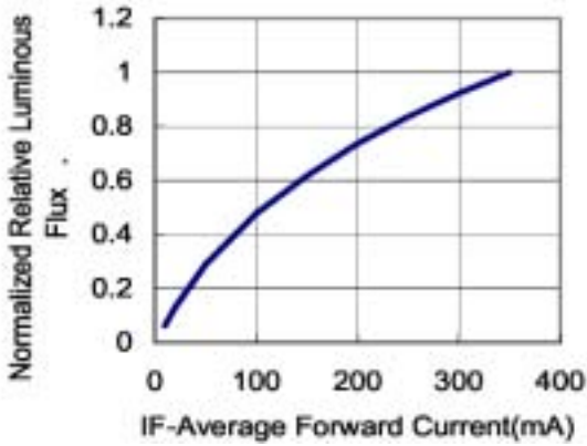
Fig 4a. Relative Luminous Flux vs. Forward Current for White, Blue and Green at T_j=25 maintained.
