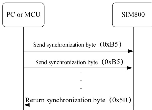
Figure 3: Synchronization word detection
