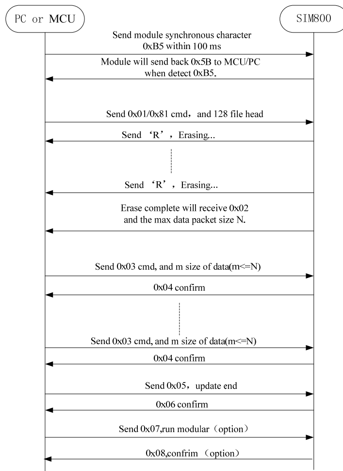
Figure 1: Upgrade process
