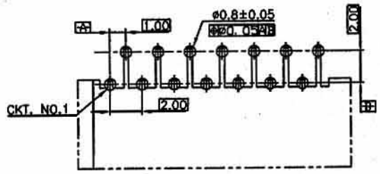
PC BOARD LAYOUT PCB T=0.6mm TOP VIEW
