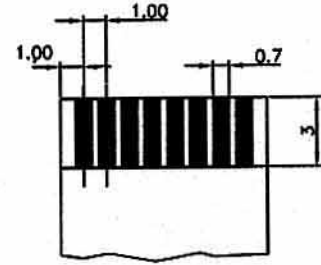
FFC/FPC DIMENSION THICKNESS 0.26~0.32mm TOLERANCE: 0.05mm
