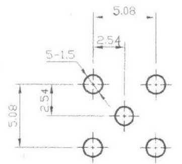
RECOMMENDED MOUNTING HOLES
