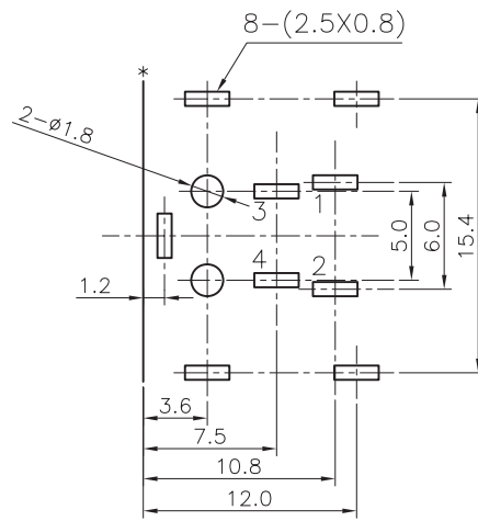
FOR 4PIN ONLY RECOMMEND PCB LAYOUT (TOLERANCE= \pm 0.05 )
